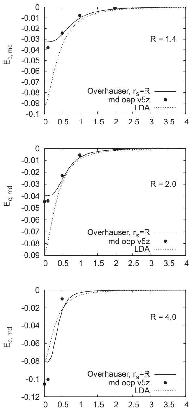
FIGURE 7. The short-range correlation energy for range-separated multideterminant DFT as a function of the cutoff parameter \mu for the \text{H}_2 molecule at three different values of the internuclear distance R . Dots (●) are “exact” values (see text in Section 6), solid lines are the results from the Overhauser model, and the dashed lines are the LDA values.
