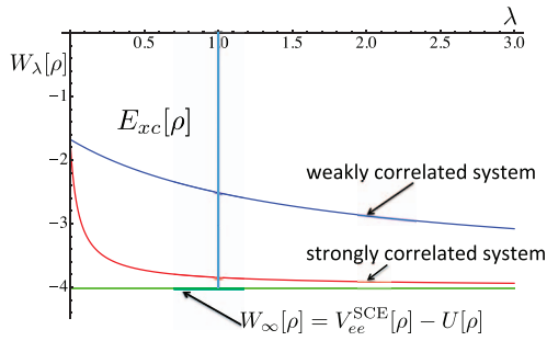
FIG. 1. The KS SCE approximation from the point of view of the adiabatic connection of Eq. (25). We have reported W_\lambda[\rho] as a function of \lambda for a typical weakly correlated and a typical strongly correlated system. The area between W_\lambda[\rho] , the \lambda -axis and the vertical lines corresponding to \lambda = 0 and \lambda = 1 gives the exchange-correlation energy E_{xc}[\rho] . The KS SCE approximates W_\lambda[\rho] with its value at \lambda \rightarrow \infty for all \lambda , and thus the xc energy with the area of the rectangle limited by W_\infty[\rho] , the \lambda -axis, and the vertical lines corresponding to \lambda = 0 and \lambda = 1 .
