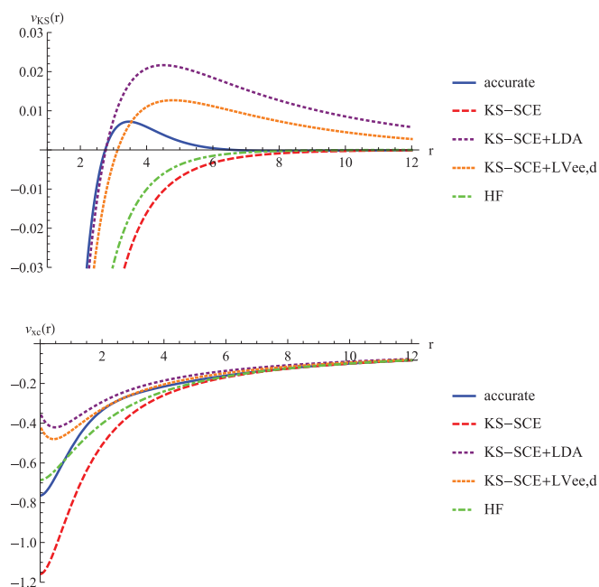
FIG. 8. v_{\text{KS}}(r) and v_{\text{xc}}(r) for \text{H}^- and various approaches.
