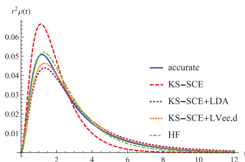
FIG. 5. r^2 \rho(r) for \text{H}^- and various approaches.
