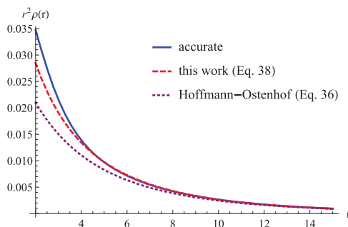
FIG. 3. Comparison of the long-range behavior of r^2\rho(r) at Z_{\text{crit}} obtained from the asymptotic decay expressions in Eqs. (36) and (38) with the almost exact result obtained from the wavefunction in Sec. II A.
