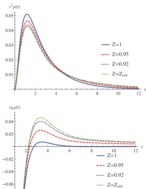
FIG. 2. Accurate r^2\rho(r) and v_{\text{KS}}(r) for various anions with nuclear charge Z of the He isoelectronic series.
