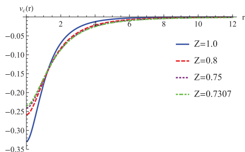
FIG. 9. The self-consistent correlation potentials v_c(r) from the bare KS SCE method.
