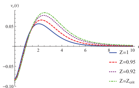
FIG. 4. Accurate correlation potential v_c(r) for various Z .
