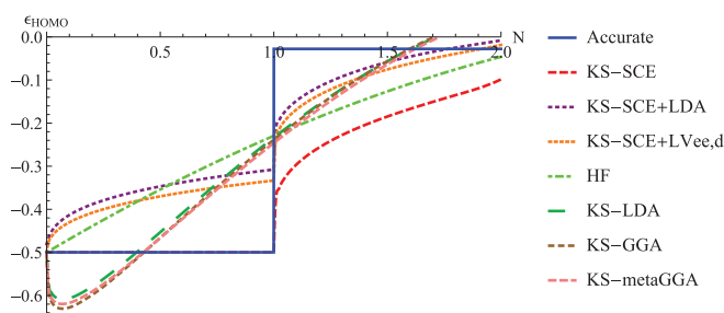
FIG. 10. \epsilon_{\text{HOMO}} vs. N in the Hydrogen nuclear potential for various approaches.
