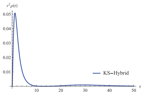
FIG. 7. r^2\rho(r) for \text{H}^- with the B3LYP functional and a ET-QZ3P plus 3 diffuse function basis. It displays a second unphysical maximum in the density.
